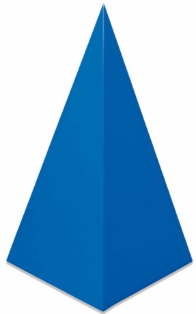
square pyramid
