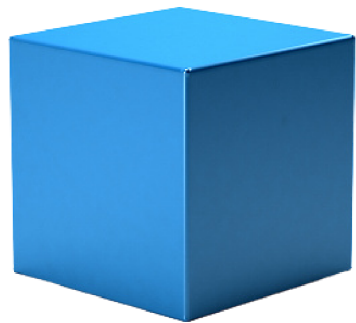
cube
